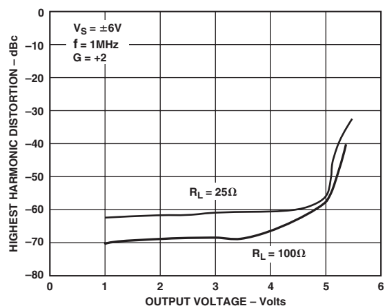
TPC 12. Distortion vs. Output Voltage, V_S = \pm 6V , G = +2 , f = 1MHz
