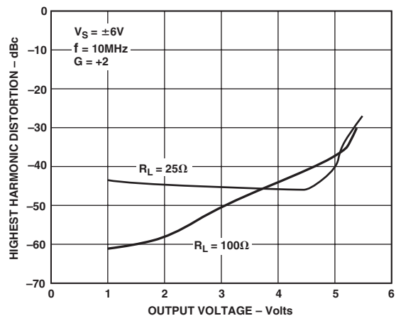
TPC 13. Distortion vs. Output Voltage, V_S = \pm 6V , G = +2 , f = 10MHz
